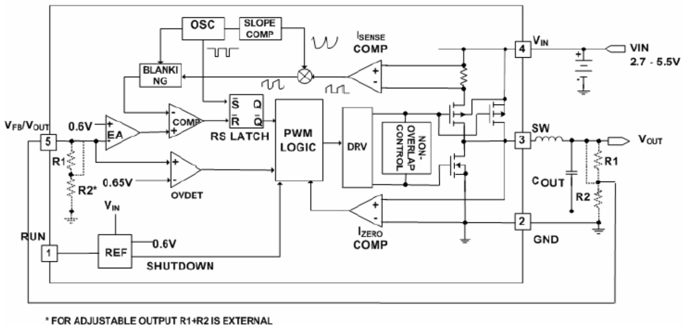
Figure 2 N6200 Block Diagram
